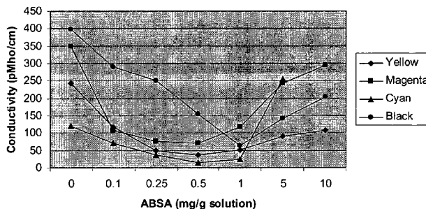
Toner bulk conductivity reduced with the amount of the addition of alkylbenzenesulfonic acid (ABSA, mixture of C 11 , C 12 and C 13 carbon chain length) in the depleted toner
